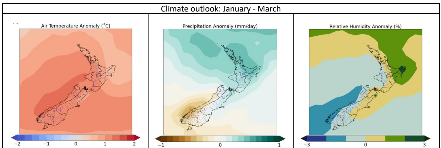
Figure 7: Climate outlook for January-March showing forecast temperature (left), rainfall (middle) and relative humidity (right) anomalies.
