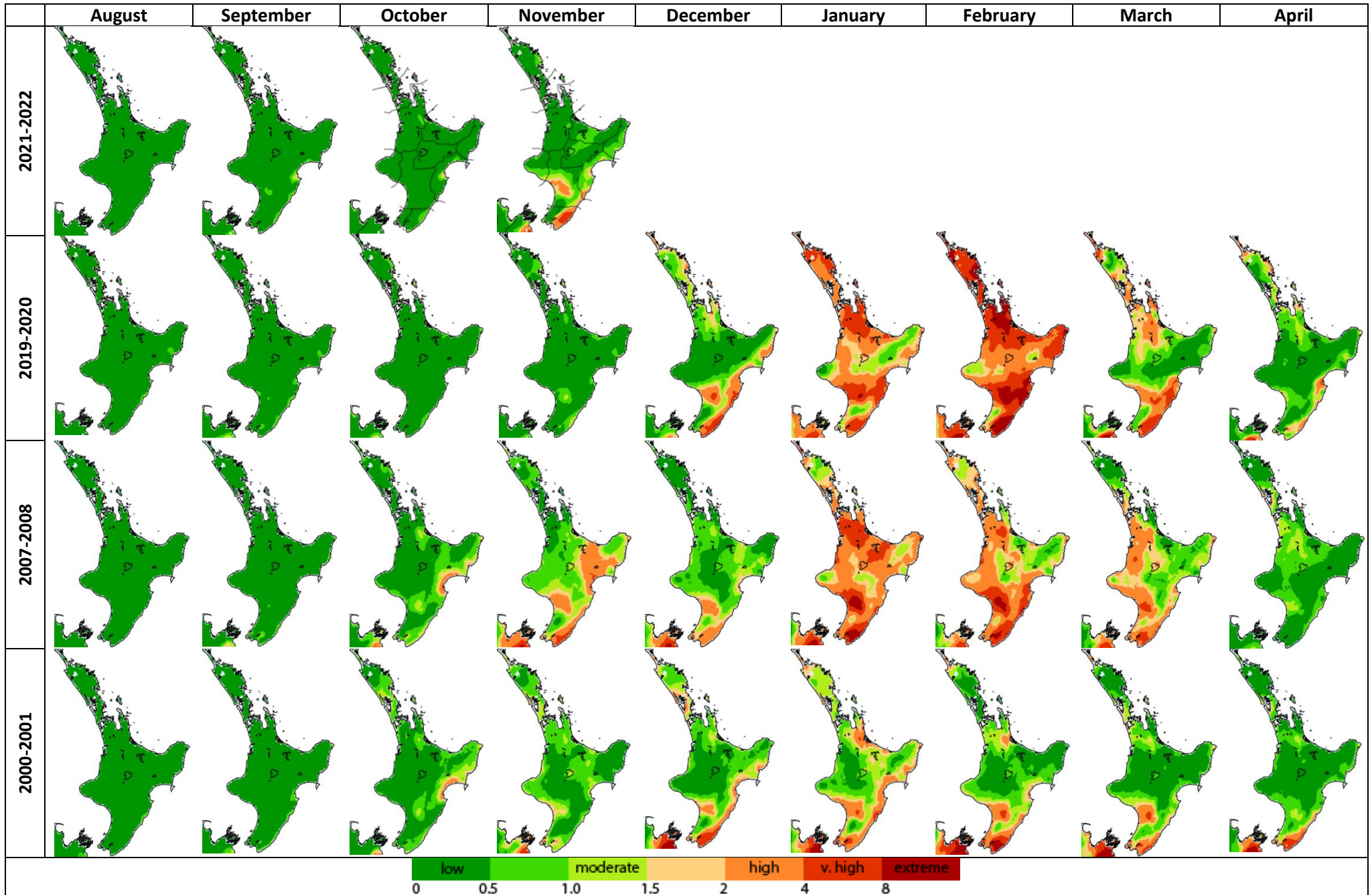
Figure 8: Monthly average severity rating for 2021-2022 up to and including November and the comparative years of 2019/2020, 2007/2008 and 2000/2001. These are analogue years for the current season and give us an insight into what the upcoming season may be like.
