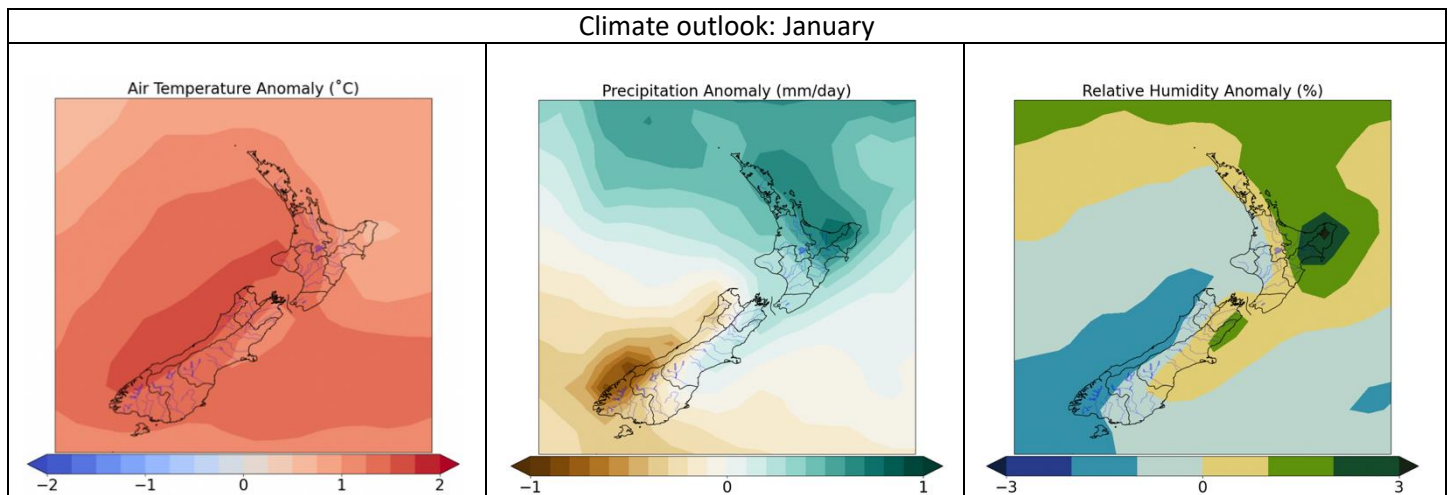
Figure 6: Climate outlook for January showing forecast temperature (left), rainfall (middle) and relative humidity (right) anomalies.
