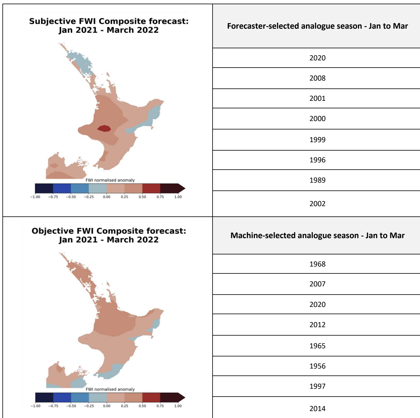
Figure 5: Analogue fire seasons as selected with expert interpretation from NIWA (top) and automated computer analysis (bottom). The fire weather index is a combination of the initial spread index and build-up index, and is a numerical rating of the potential frontal fire intensity. In effect, it indicates fire intensity by combining the rate of fire spread with the amount of fuel being consumed. Here, the fire weather index anomaly is calculated by averaging historical analogue years together and comparing to the average fire weather index between 1991-2020 for the relevant season.
