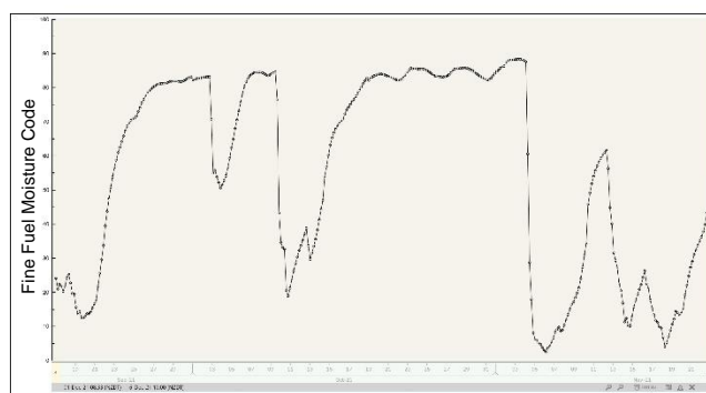
Figure 2: Graph of hourly Fine Fuel Moisture Code values for the past month based on observed weather for the Napier Raws.
